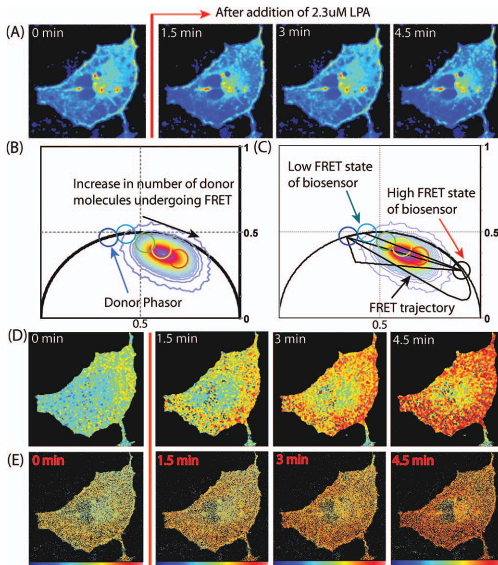
Fig. 5. FRET detection of a RhoA-kRas single chain biosensor, with constitutive membrane localization. A: Intensity images of COS7 cell transfected with (RBD-Citrine)-1L-(ECFP-RhoA-kRas) before and after LPA stimulation (donor channel). B: Phasor plot of (RBD-Citrine)-1L-(ECFP-RhoA-kRas) experiment. C: FRET efficiency
