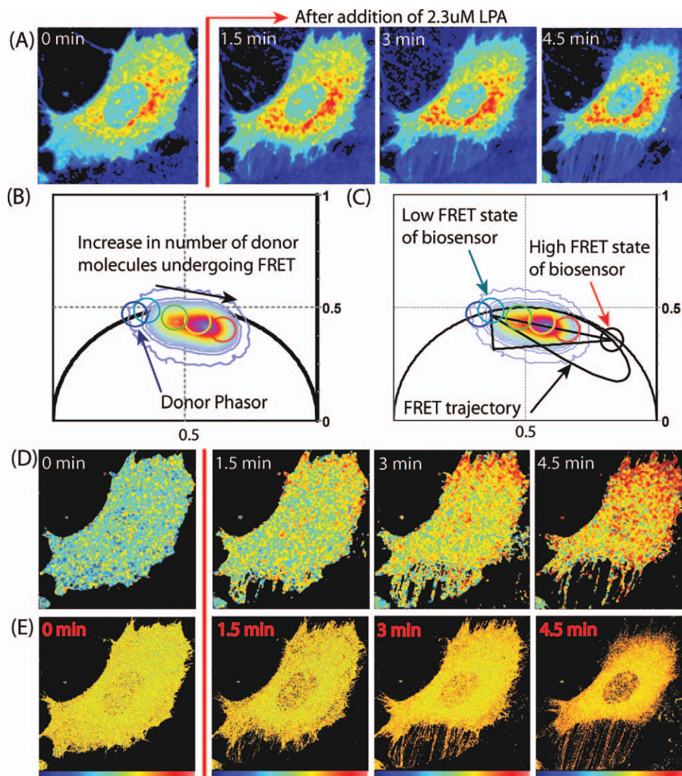
Fig. 4. FRET detection of a single chain RhoA biosensor, with normal subcellular localization. A: Intensity images of COS7 cell transfected with (RBD-Citrine)-1L-(ECFP-RhoA) before and after LPA stimulation (donor channel). B: Phasor plot of (RBD-Citrine)-1L-
